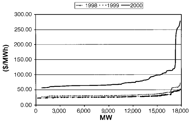
FIGURE 1. CALIFORNIA FOSSIL-FUEL PLANTS MARGINAL COST CURVES, SEPTEMBER
